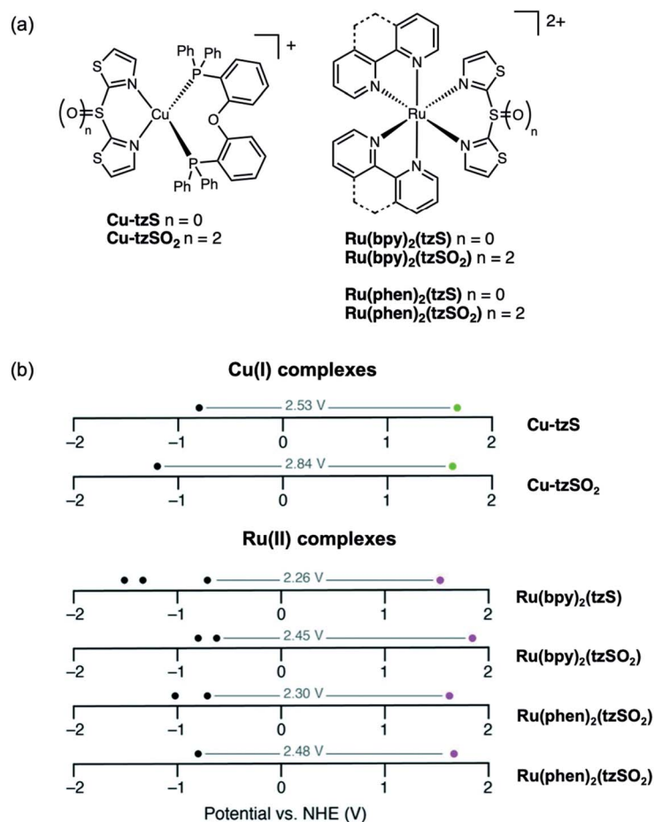
Fig. 19 (a) Structures of Cu-tzSO n and Ru(bpy) 2 (tzSO n ) and Ru(phen) 2 (tzSO n ) complexes reported by our group (n = 0, 2). (b) Redox potentials of Cu(I) and Ru(II) complexes with reductive (black dots) and oxidative (green or purple dots) potentials illustrated. Adapted with permission from ref. 95. Copyright 2019 Royal Society of Chemistry.
