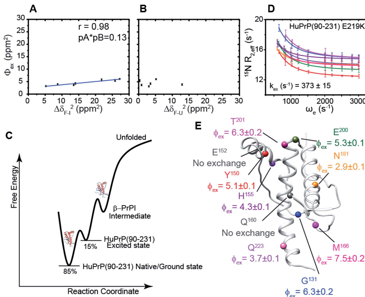
Fig. 6 Correlation between relaxation dispersion/thermal unfolding data. (A and B) \Phi_{\text{ex}} parameters (ppm 2 ) derived from the global fit of cluster A ( k_{\text{ex}} = 2502 \pm 106 \text{ s}^{-1} ) of HuPrP(90–231) plotted as a function of the squared differences in chemical shift between the native and the intermediate state ( \Delta\delta_{\text{F-I}}^2 ) (ppm 2 ) (A) and between the native and the denaturated state ( \Delta\delta_{\text{F-U}}^2 ) (ppm 2 ) (B). (C) Conformational landscape of HuPrP(90–231) revealed by NMR relaxation dispersion and thermal melt data. (D) Best fit curves to a two-site exchange model assuming a common motion for residues of HuPrP(90–231) E219K. (E) Mapping of the residue-specific \Phi_{\text{ex}} parameters extracted for HuPrP(90–231) E219K from the global fit. The residues that do not show any RD profile are reported as dark grey spheres.
