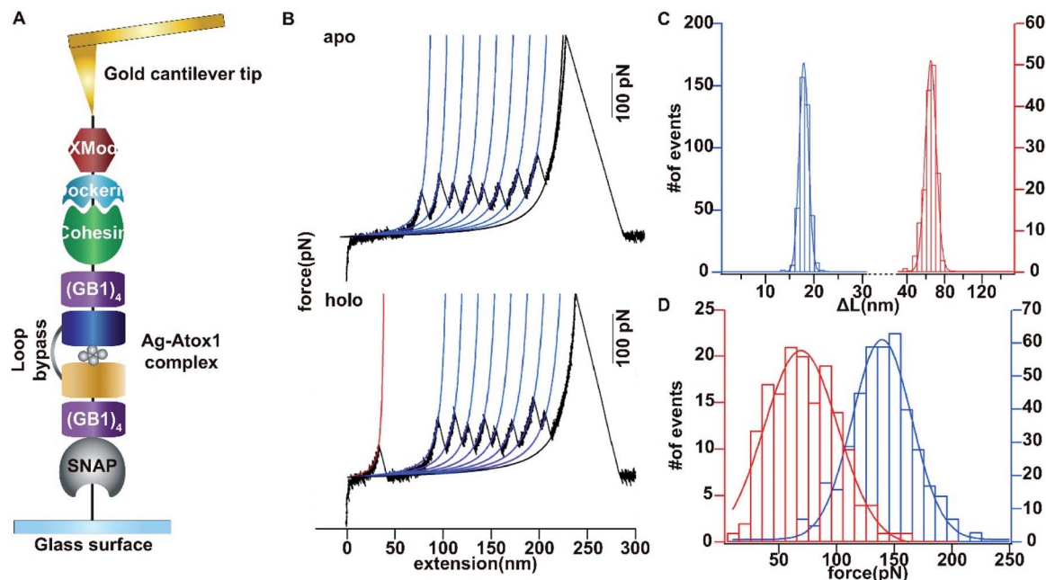
Fig. 1 Single-molecule force spectroscopy analysis of the mechanical stability of the \text{Ag}_4-(\text{Atox1})_2 complex. (A) Depiction of the experimental pulling configuration, with XMod-Doc attached to the gold cantilever tip and Coh-(GB1) 4 -Atox1-linker-Atox1-(GB1) 4 -SNAP-tag attached to the glass surface. (B) Single-molecule force spectroscopy experiments on the engineered chimeric polyprotein in the absence and presence of Ag. The representative force-extension traces for the stretching of the polyprotein in the apo and holo forms are shown. (C) The distributions of contour length increments for the stretching of the polyprotein in the apo and holo forms are shown respectively. Given that Atox1 and the linker comprise 68 and 54 amino acids, respectively, and the N-C distance of the structured Atox1-Ag-Atox1 complex is 5.6 nm, the contour length increment is expected to be 63.75 nm ((68 aa \times 2 + 54 aa) \times 0.365 nm/aa – 5.6 nm). (D) The unfolding force histogram for the stretching of the polyprotein in the apo and holo forms is shown respectively.
