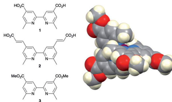
Fig. 7 Structures of ligands 1–3, and the structure of [\text{Cu}(\text{3})_2]^+ in the [\text{PF}_6]^- salt (CSD refcode JOHXIO). The space-filling representation is used to emphasize the protection imparted by the 6- and 6'-methyl groups.
