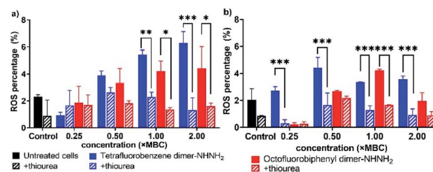
Fig. 6 Reactive oxygen species generated from (a) A. baumannii , and (b) MDR-FADDI-AB156 under treatment of tetrafluorobenzene dimer-NHNH 2 6 and octofluorobiphenyl dimer-NHNH 2 7 . The flow cytometric graphs are provided in Fig. S10 and S11.† All data are expressed as mean ± standard deviation as indicated by the error bars ( n = 4 ). * P \leq 0.05 , ** P \leq 0.01 , *** P \leq 0.001 . Student's t -test, a significant difference from thiourea quenched ROS control.
