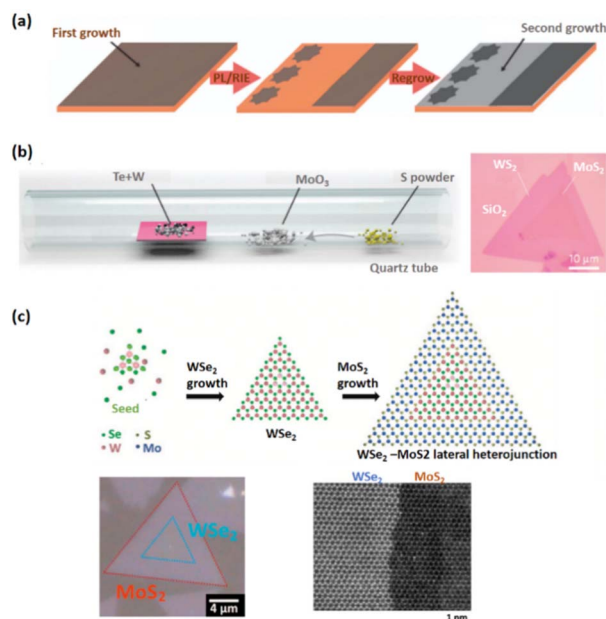
Fig. 5 Shows the 2D lateral heterostructures grow in-plane epitaxially. (a) Schematic depiction of the CVD developing process for graphene/h-BN lateral heterojunctions. 86 Reprinted from ref. 86 with permission from Nature, copyright 2012. (b) Optical image of the WS_2/MoS_2 lateral heterostructures and schematic representation of the one-pot synthesis setup. 89 Reprinted from ref. 89 with permission from Nature, copyright 2014. (c) The optical picture of the monolayer WSe_2/MoS_2 lateral heterojunction, as well as its two-step production. The comparable high-resolution STEM pictures taken at the interface are shown on the right. 90 Reprinted from ref. 90 with permission from The American Association for the Advancement of Science (AAAS), copyright 2015.
