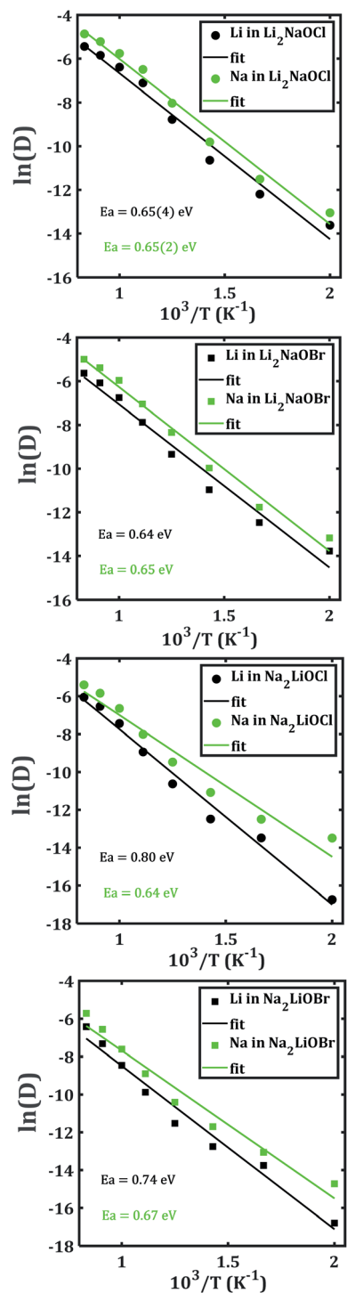
Fig. 6 Arrhenius dependence of Li + and Na + diffusion coefficient ( D ) of Li 2 NaOX and Na 2 LiOX structures.
