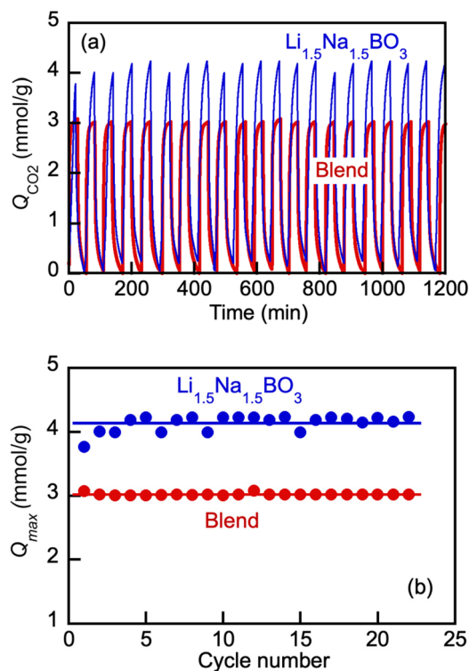
Fig. 8 Effect of cycling on \text{CO}_2 uptake by molten Li, Na borate ( \text{Li}_{1.5}\text{Na}_{1.5}\text{BO}_3 ) and eutectic Li, K carbonate ( \text{Li}_{1.24}\text{K}_{0.76}\text{CO}_3 ) blend (borate/carbonate ratio, 1 : 1 mol/mol) (a) and maximum \text{CO}_2 loading in each cycle at t_{\text{cycle}} = 30 \text{ min} ( Q_{\text{max}} , \text{mmol g}^{-1} ) vs. cycle number (b). Cycling was conducted via pressure swing operation on repeated switching of the gas stream between 100% \text{CO}_2 ( p_{\text{CO}_2} = 1 \text{ bar} ) and 100% \text{N}_2 ( p_{\text{CO}_2} = 0 \text{ bar} ) at 550 ^\circ\text{C} . Cycle consisted of alternating 30 min of \text{CO}_2 flow followed by nitrogen flow ( 60 \text{ mL min}^{-1} ) for 30 min. The salt samples (6 mg) were evenly spread at the bottom of a platinum pan; temperature 550 ^\circ\text{C} throughout.
