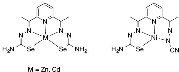
Fig. 16 Examples of complexes with multidentate selenoacetylpyridine ligands.
