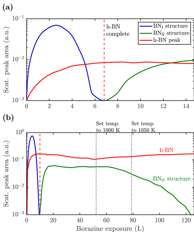
Fig. 5 Peak areas of the characteristic diffraction peaks representing the different structures versus borazine exposure. After the \text{BN}_I structure has disappeared the h-BN peak saturates giving rise to a conversion and further exposure leads to the rise of the \text{BN}_{II} structure. Due to a higher substrate temperature of 915 K in (a), the \text{BN}_I structure disappears already after an exposure of \approx 7 L compared to 10 L at 880 K in (b), thus indicating a kinetically driven conversion. Dosing in (b) is then further continued with subsequent changes of the surface temperature as stated above the diagram. After long enough exposure the \text{BN}_{II} structure disappears leaving a strong h-BN intensity behind.
