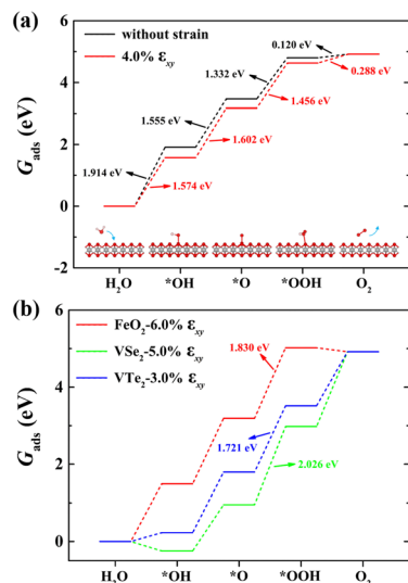
Fig. 2 Gibbs free energy diagrams of the adsorbed intermediates for the OER on (a) monolayer CoO 2 without strain and under 4.0% biaxial tensile strain, and (b) monolayer FeO 2 , VSe 2 or VTe 2 under 6.0%, 5.0% and 3.0% biaxial tensile strain, respectively. The inset in (a) shows the reaction steps in which the O*, OH* and OOH* intermediates adsorb on monolayer CoO 2 , where the red, gray and white spheres denoted O, Co and H atoms, respectively.
