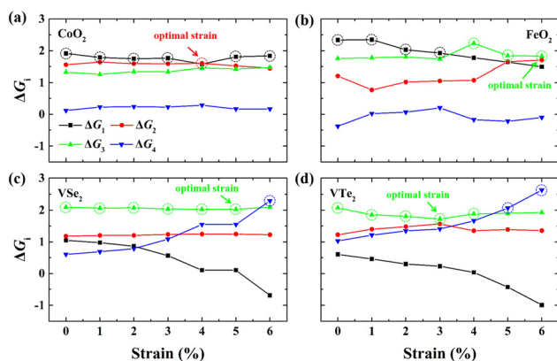
Fig. 3 Gibbs free energy differences ( \Delta G_i ) in the elementary reaction steps for (a) CoO 2 , (b) FeO 2 , (c) VSe 2 and (d) VTe 2 monolayers under different biaxial tensile strains. The PDSS are circled by dash lines and the optimal strains for the lowest overpotentials are marked by arrows.
