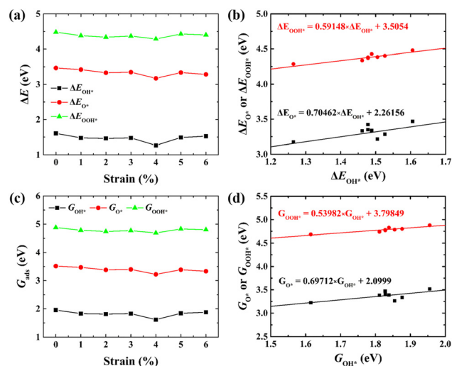
Fig. 4 (a) Binding energies of the three intermediates on the CoO 2 monolayer under different biaxial tensile strain, and (b) the scaling relation between \Delta E_{OH^*} and \Delta E_{O^*} or \Delta E_{OOH^*} . (c) Adsorption Gibbs free energies of the three intermediates on CoO 2 under different biaxial tensile strain, and (d) the scaling relations between G_{OH^*} and G_{O^*} or G_{OOH^*} . The solid lines in (b) and (d) are fitting lines.
