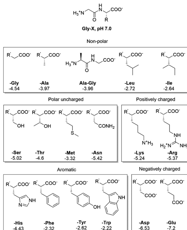
Fig. 5 Structure of side chains of Gly-X dipeptides and their log D values (more negative log D values correspond to a higher hydrophilicity). R' = \text{H}_3\text{N}^+ - \text{CH}_2 - \text{CONH} - \{
