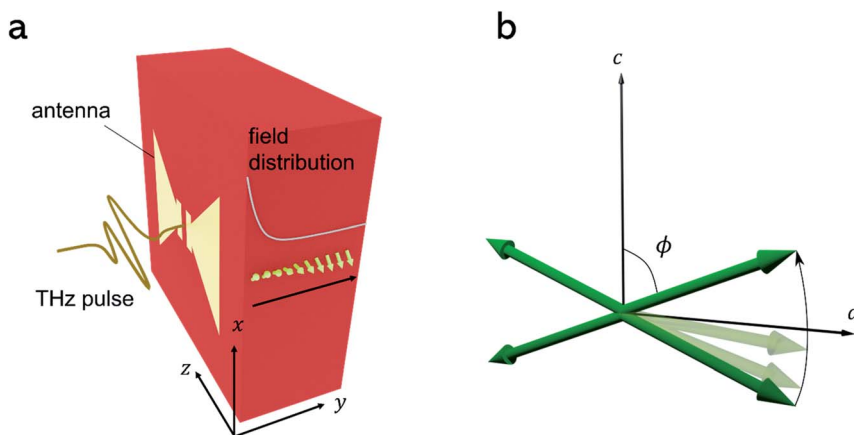
Fig. 1 Model structure for simulation. (a) The THz field is enhanced with metallic antenna fabricated on top of the orthoferrite crystal \text{TmFeO}_3 . The incident pulse travels in the sample from the antenna side. Exponentially localised evanescent field induces spin switching and generates spin waves. (b) There are four stable positions for antiferromagnetic vector \mathbf{G} in the \Gamma_{24} phase, especially four-fold symmetric placement in the midpoint between T_1 and T_{\text{u}} . Through switching by external stimulation, the \mathbf{G} jumps to another stable state in the ac -plane.
