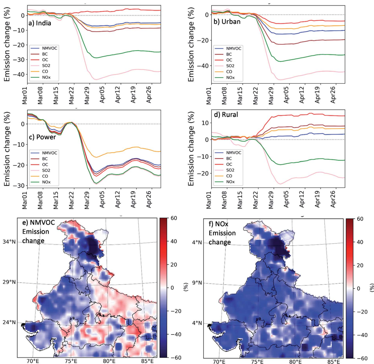
Fig. 2 Daily emission change due to AF applied on CEDS_M emissions averaged in (a) India, (b) Urban, (c) Power, and (d) Rural (X-axis shows the days in March and April and the Y-axis range is different for each subplot). Map of emission changes of (e) NMVOC and (f) NO x averaged in April 2020. The location of the box regions can be found in the ESI.†
