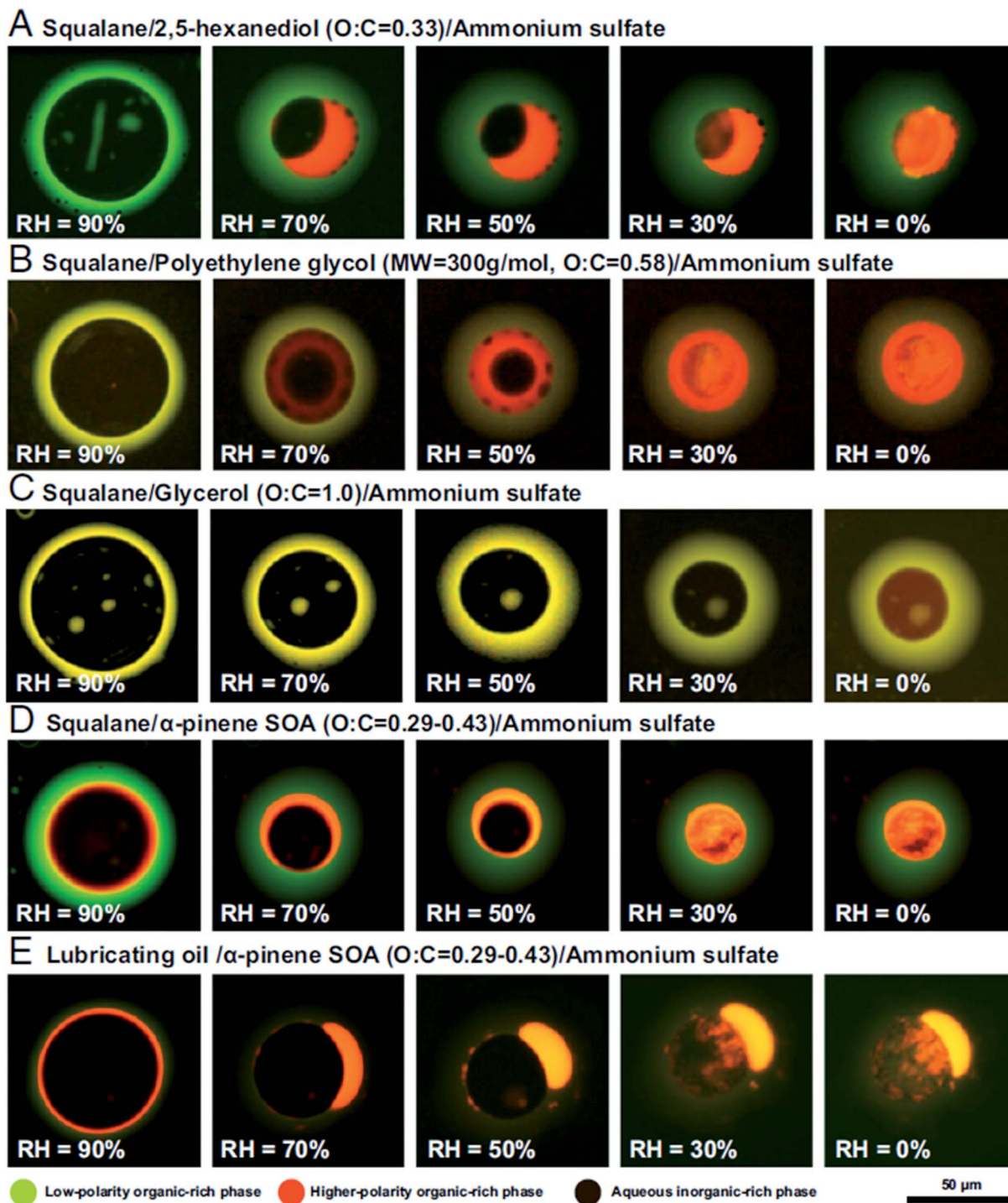
Fig. 4 Fluorescence microscopy images of single particles containing proxies for primary organic aerosol (green), secondary organic aerosol (orange), and secondary inorganic aerosol (black) as a function of relative humidity. Compositions are indicated above each row. The coloring is due to trace amounts of Nile red dye. The scale bar applies to all images. Reprinted from ref. 151 under a CC BY-NC-ND License 4.0 ( https://creativecommons.org/licenses/by-nc-nd/4.0/ ).
