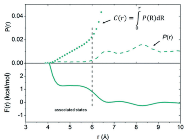
Fig. 2 Free energy curve, F(r) , and probability distribution, P(r) , computed from MD simulations of P^t(\text{Bu})_3/\text{B}(\text{C}_6\text{F}_5)_3 in toluene. Reproduced from ref. 67 with permission from the Royal Society of Chemistry.
