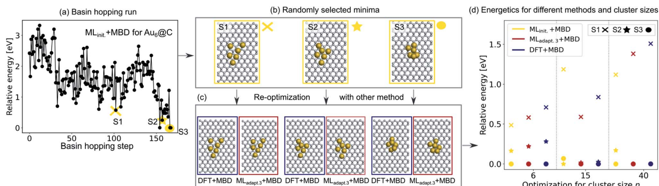
Fig. 4 (a) Basin hopping run with ML_{init.} for Au@C with Au 6 nanoclusters (NCs). Yellow circles indicate (b) 3 selected structures S1–S3 that include the energetically lowest geometry and two randomly selected structures according to ML_{init.} that are (c) reoptimized with DFT+MBD (blue) and ML_{adapt,3} +MBD (red). (d) Relative energies reported with respect to the energetically lowest cluster for each method. In addition, energy rankings of the energetically lowest structures and two randomly selected structures from basin hopping runs with NC sizes of 15 and 40 atoms using ML_{init.} +MBD (yellow), ML_{adapt,3} +MBD (red), and DFT+MBD (blue). Corresponding structures are shown for each method in Fig. S2.†
