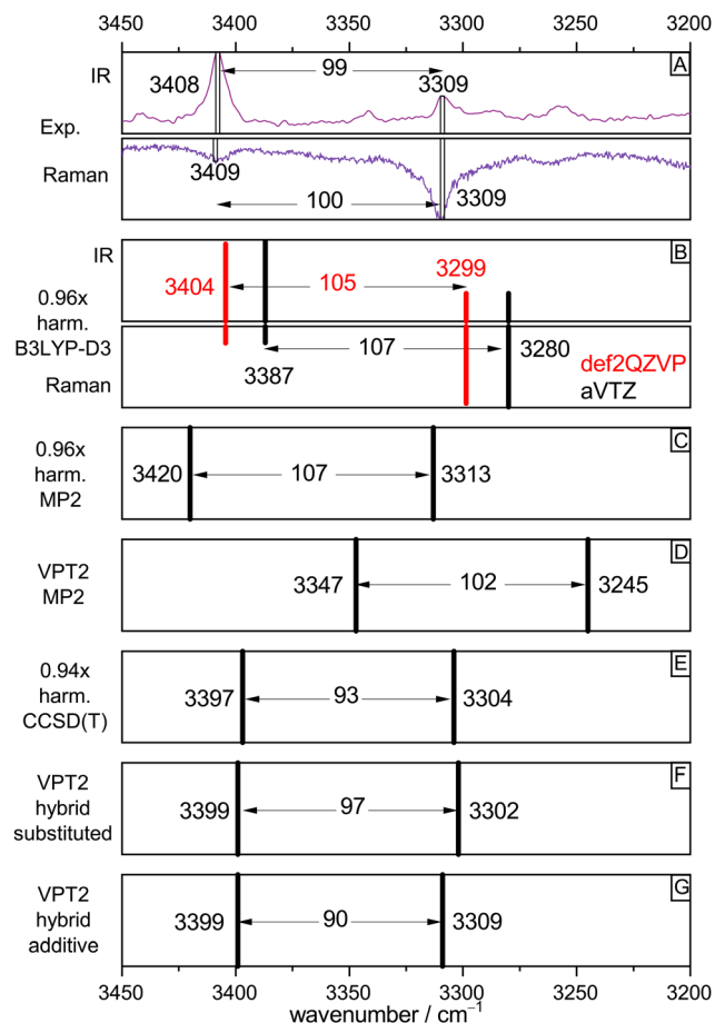
Fig. 4 Comparison of experimental OH stretching band positions (from Fig. 2, trace c, IR and Fig. 3, trace c, Raman) and their splitting with harmonic and anharmonic predictions for the (T_g^t F) dimer. See text for explanations.
