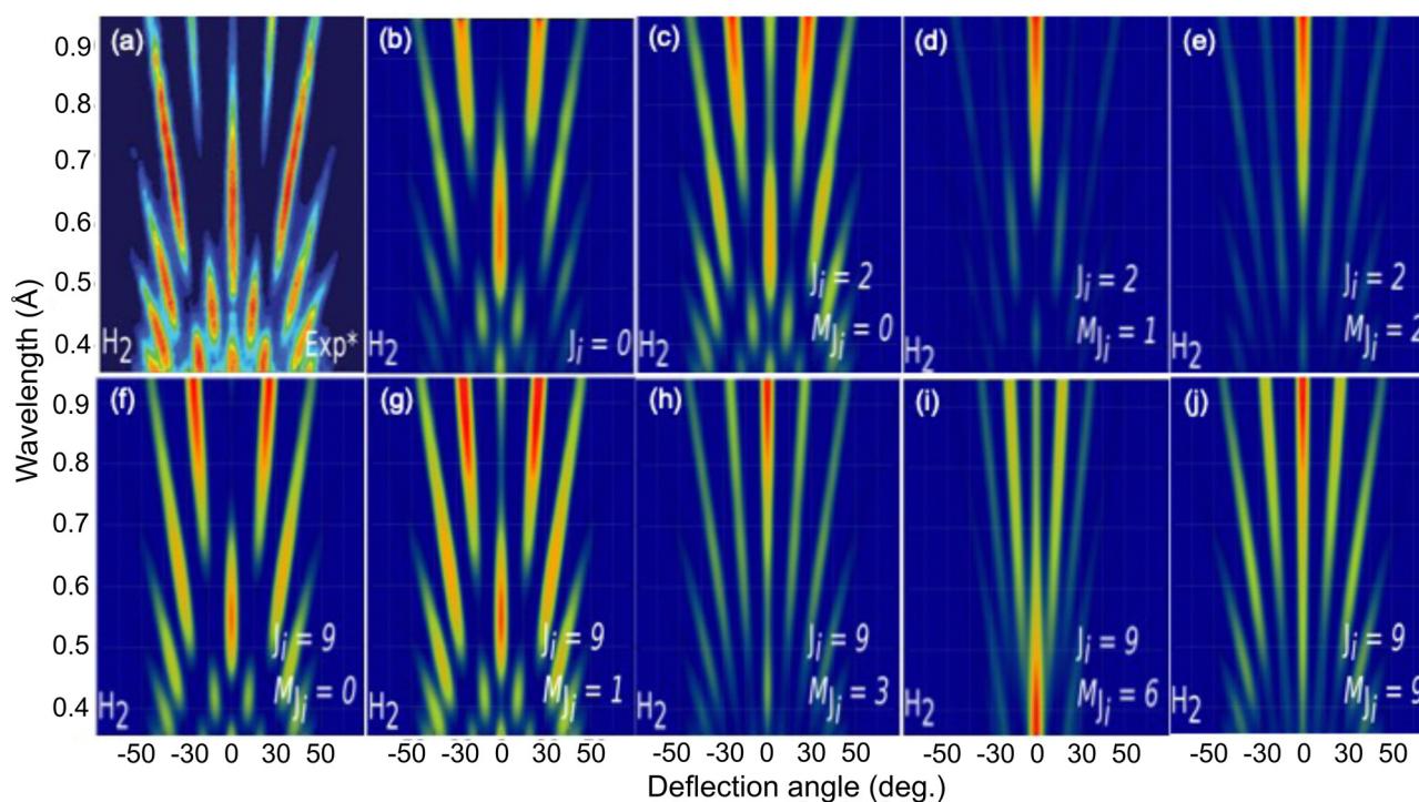
Fig. 6 \text{H}_2/\text{KCl}(001) GIFMD patterns along the crystallographic direction [100]. (a) Experimental pattern (data taken from ref. 67); (b), (c), (d), (e), (f), (g), (h), (i) and (j) simulated pattern for (J = 0, M_J = 0) , (J = 2, M_J = 0) , (J = 2, M_J = 1) , (J = 2, M_J = 2) , (J = 9, M_J = 0) , (J = 9, M_J = 1) , (J = 9, M_J = 3) , (J = 9, M_J = 6) and (J = 9, M_J = 9) , respectively.
