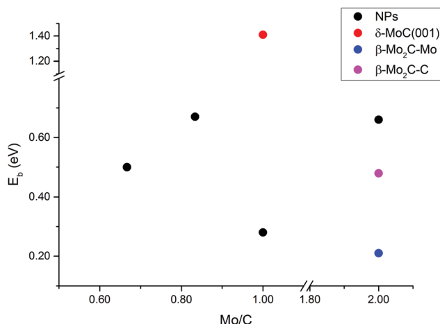
Fig. 9 Energy barrier ( E_p ) for CO 2 dissociation on nanoparticles (NPs) at different Mo/C ratios. Data of \delta -MoC(001) and \beta -Mo 2 C(001) surfaces are included for comparison. \beta -Mo 2 C(001) Mo- and C-terminations are shown as \beta -Mo 2 C–Mo and \beta -Mo 2 C–C, respectively.
