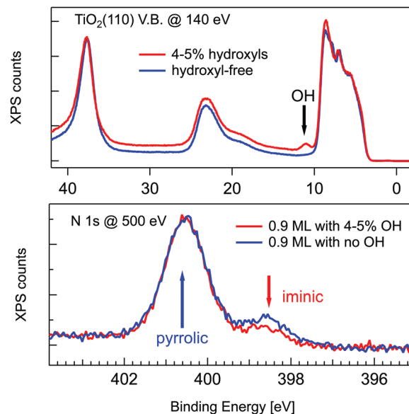
Fig. 4 Upper panel: Valence band photoemission from a slightly hydroxylated (red line) and a hydroxyl-free surface (blue line) before deposition; the OH 3σ peak is marked with an arrow. Lower panel: Photoemission spectra of the N 1s peak for 0.9 ML of 2H-TTP deposited at RT on the same surfaces of the upper panel. Reproduced from ref. 47 with permission from the American Chemical Society, Copyright 2017.
