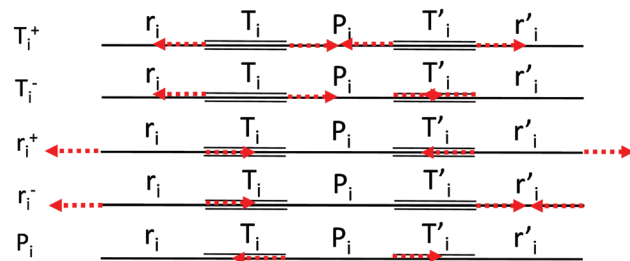
Fig. 2 Definition of the CC stretching internal coordinates and sketches of their symmetry adapted combinations \{S_x\} .
