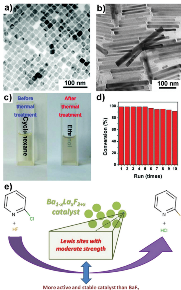
Fig. 6 TEM images of (a) NaScF 4 and (b) KSc 2 F 7 nanocrystals. (c) Photograph of NaScF 4 nanocrystal solutions before and after thermal treatment at 500 °C under Ar/H 2 . (d) Reusability test of NaScF 4 nanocrystals for 10 cycles in the cyanosilylation reaction. 96 Reprinted with permission from ref. 96. Copyright 2017, Royal Society of Chemistry. (e) A scheme for the gas phase fluorination of 2-chloropyridine by HF using Ba 1-x La x F 2+x . 97 Reprinted with permission from ref. 97. Copyright 2017, Elsevier.
