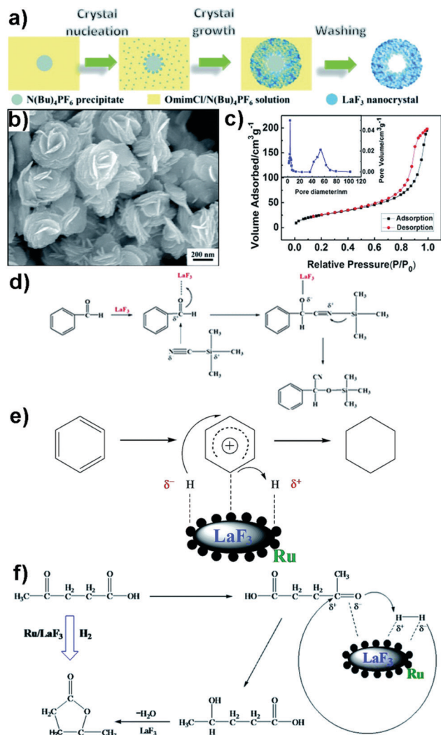
Fig. 5 (a) A scheme for the formation of hollow mesoporous ReF 3 (Re is La, Nd, or Y) nanocrystals. (b) SEM image of mesoporous LaF 3 nanocrystals. (c) Nitrogen adsorption and desorption isotherms of mesoporous LaF 3 nanocrystals shown in (b) (pore-size distribution is included in the inset). (d) Proposed reaction mechanism for the cyanosilylation reaction catalysed by LaF 3 . (e) Proposed reaction mechanism for the benzene hydrogenation to cyclohexane using the co-catalyst Ru/LaF 3 . (f) Proposed reaction mechanism for levulinic acid (LA) hydrogenation to γ-valerolactone using the co-catalyst Ru/LaF 3 . 95 Reprinted with permission from ref. 95. Copyright 2015, Royal Society of Chemistry.
