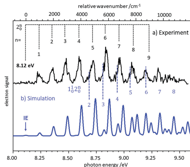
Fig. 3 Slow photoelectron spectrum of BH 2 (upper trace) compared with a Franck–Condon simulation. The IE was derived from the best agreement between experiment and simulation. Figure taken from ref. 61 by permission of the RSC.
