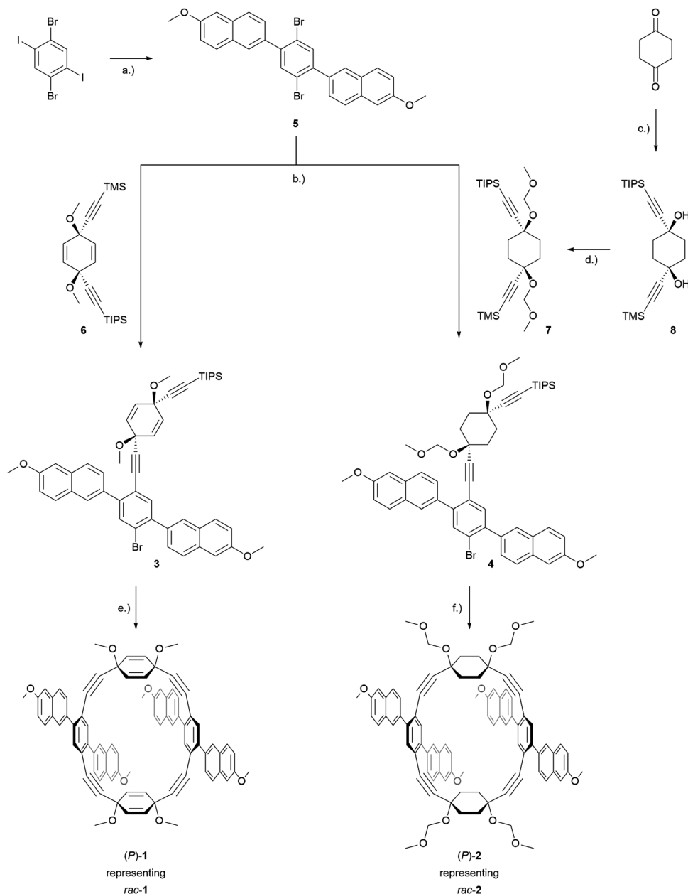
Scheme 2 Synthesis of rac -1 and rac -2. Reagents and conditions: (a) 6-methoxy-2-naphthaleneboronic acid, \text{K}_2\text{CO}_3 , \text{Pd}(\text{PPh}_3)_4 , toluene/ethanol/water (4 : 1 : 1), 90 °C, 16 h, 80%; (b) (1) \text{K}_2\text{CO}_3 , MeOH, 1–2 h; (2) \text{Pd}(\text{PPh}_3)_4 , CuI, THF/piperidine (3 : 1), 80 °C, 3–16 h, 37% for 3 , 22% for 4 (c) (1) \text{CeCl}_3 , LiCl, THF, rt, 2 h; (2) (Triisopropylsilyl)acetylene, n -BuLi, THF, –78 °C, 4 h; (3) Ethynyltrimethylsilane, n -BuLi, THF, –78 °C, 16 h, 25%; (d) \text{Pr}_2\text{NEt} , methoxymethyl chloride, \text{CH}_2\text{Cl}_2 , 16 h, 71%; (e) (1) TBAF, THF, 1 h; (2) \text{Pd}(\text{PPh}_3)_4 , CuI, THF/ \text{NEt}_3 (3 : 1, 4 mM), 14%; (f) (1) TBAF, THF, 1 h; (2) \text{Pd}(\text{PPh}_3)_4 , CuI, THF/piperidine (3 : 1, 1 mM), 17%.
