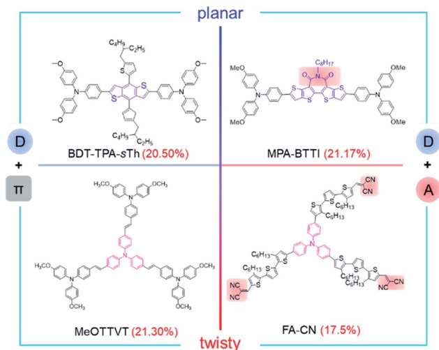
Fig. 10 Excellent photovoltaic performance of PSCs based on dopant-free HTMs with different molecular configurations and electronic properties. 37,67,132,136
