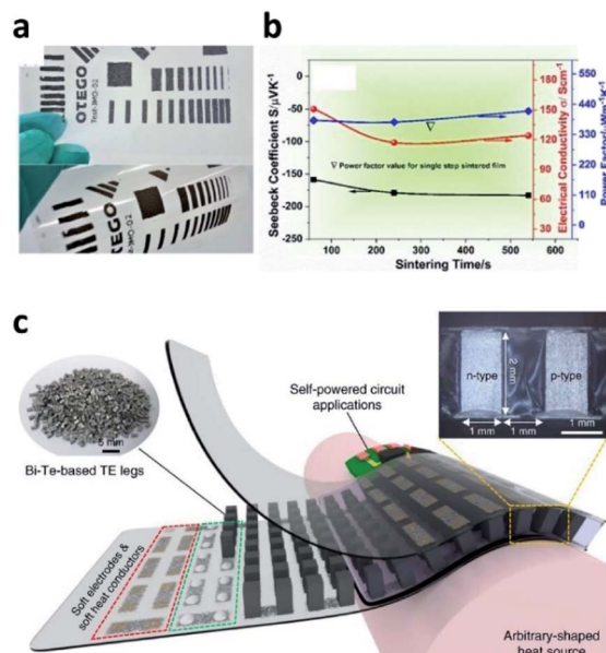
Fig. 11 (a) Flexible film on PET produced via screen printing. (b) Variation of \sigma , S , and S^2\sigma vs. sintering time. Reproduced from ref. 127 with permission from American Chemical Society. (c) Schematic of a flexible thermoelectric generator (TEG). Reproduced from ref. 135 with permission from John Wiley and Sons.
