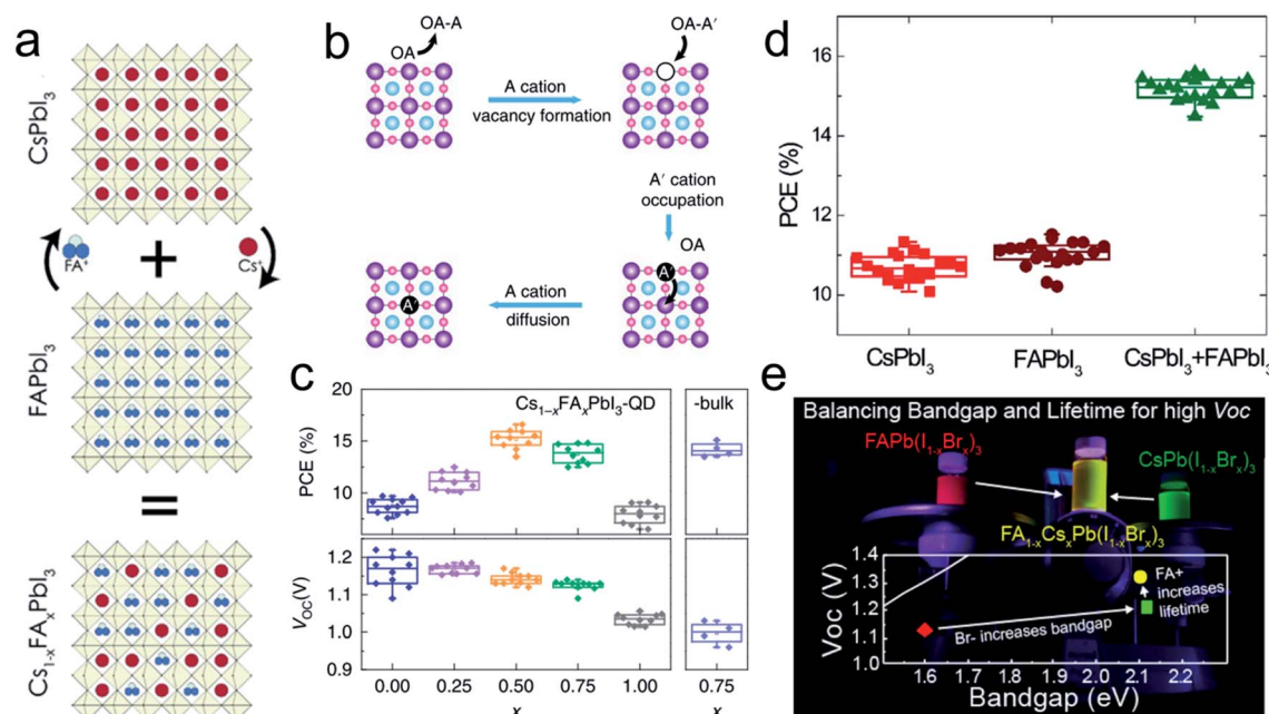
Fig. 4 A-site regulation for AIPQDSCs. (a) Schematic diagram of the cross-exchange of \text{Cs}^+ and \text{FA}^+ ions between \text{CsPbI}_3 and \text{FAPbI}_3 perovskite NCs. Adapted with permission from ref. 47 Copyright 2018, American Chemical Society. (b) A-site cation-exchange reaction mechanism. Adapted with permission from ref. 38 Copyright 2020, Nature Publishing Group. (c) Performance of SC based on \text{Cs}_{1-x}\text{FA}_x\text{PbI}_3 QDs of different compositions. (d) Distribution of PCE of SCs based on pure \alpha - \text{CsPbI}_3 , pure \text{FAPbI}_3 , and stacked \alpha - \text{CsPbI}_3/\text{FAPbI}_3 QD. Adapted with permission from ref. 48 Copyright 2019, American Chemical Society. (e) V_{\text{oc}} versus bandgap of \text{FA}_{1-x}\text{Cs}_x\text{Pb}(\text{I}_{1-x}\text{Br}_x)_3 PQDSC. Adapted with permission from ref. 49 Copyright 2019, American Chemical Society.
