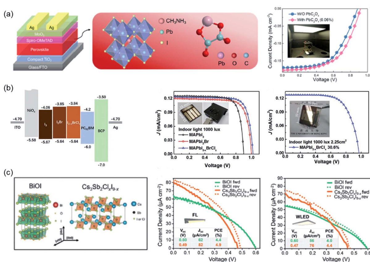
Fig. 5 (a) Schematic diagram of PSCs fabricated with PbC 2 O 4 doping and the J–V curves of with/without PbC 2 O 4 -based devices. Reproduced from ref. 201 with permission from the [American Chemical Society], copyright [2020]. (b) The bandgap of MAPbI 3 , MAPbI 2 Br, and MAPbI 2-x BrCl x perovskite and J–V curves of PSCs under indoor light conditions. Reproduced from ref. 202 with permission from the [Wiley-VCH], copyright [2019]. (c) The crystal structure of BiOI and Cs 3 Sb 2 Cl 4 I 9-x and the J–V curves of the corresponding device under FL and WLED illuminations. Reproduced from ref. 205 with permission from the [Wiley-VCH], copyright [2020].
