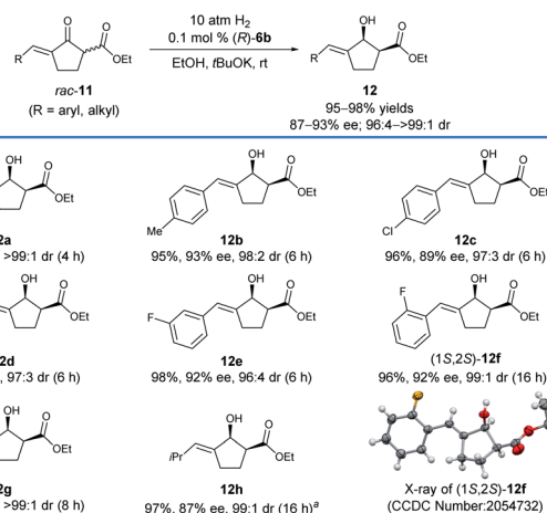
Scheme 6 Asymmetric hydrogenation of exocyclic enone esters bearing a five-membered ring, 11 . Reaction conditions: 1.0 mmol scale, 11 /tBuOK/( R )- 6b = 1000 : 10 : 1, EtOH (4.0 mL), 25–30 °C, 4–16 h. The yields are isolated yields of cis - and trans -isomers of 12 . The enantiomeric excesses (ee) of the major diastereomer and the diastereomeric ratio (dr) values were determined by HPLC analysis using a chiral column. a With ( R )- 6g as the catalyst.
