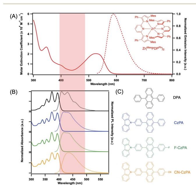
Fig. 2 (A) Electronic absorption (solid line) and photoluminescence (dashed line) spectra of Zr(MesPDP Ph ) 2 in THF. (B) Normalized absorption (solid lines) and photoluminescence (dashed lines) spectra of DPA (black), CzPA (blue), F-CzPA (green) and CN-CzPA (orange). The red shaded area shows a small spectral overlap between photoluminescence of acceptors and absorbance of Zr(MesPDP Ph ) 2 , indicating minimal reabsorption of upconverted fluorescence by the sensitizer. (C) Chemical structures of DPA (black), CzPA (blue), F-CzPA (green) and CN-CzPA (orange).
