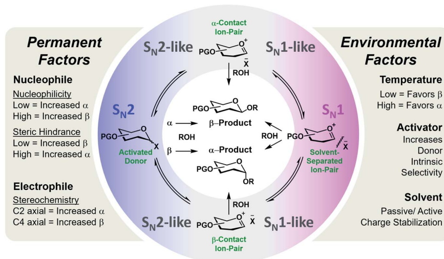
Fig. 1 General representation of the potential mechanistic pathways of glycosylations leading to either the \alpha ( \alpha ) or \beta ( \beta ) anomer of the formed C–O bond. The empirically-derived permanent and environmental factors and their influence on stereoselectivity are provided. 24
