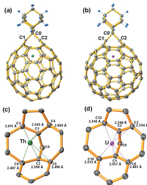
Fig. 6 ORTEP drawings of (a) \text{Th}@C_{3v}(8)-C_{82}\text{Ad(I)} and (b) \text{U}@C_{2v}(9)-C_{82}\text{Ad(I)} showing thermal ellipsoids at the 50% probability level. (c and d) The view showing the interaction of the metal ion with the closest cage portion.
