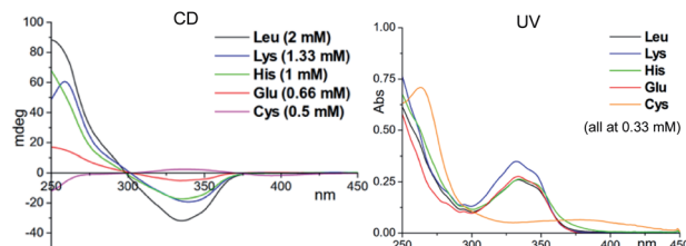
Fig. 2 Substrate scope at a normal concentration range. Standard assaying conditions (1.2 equiv. of reagents, 1 min). (A) \alpha AA and other chiral amines; a) see the ESI† for LC-MS analysis of the reaction mixture. (B) Selected CD and UV spectra; b) samples were measured at the concentration specified.
