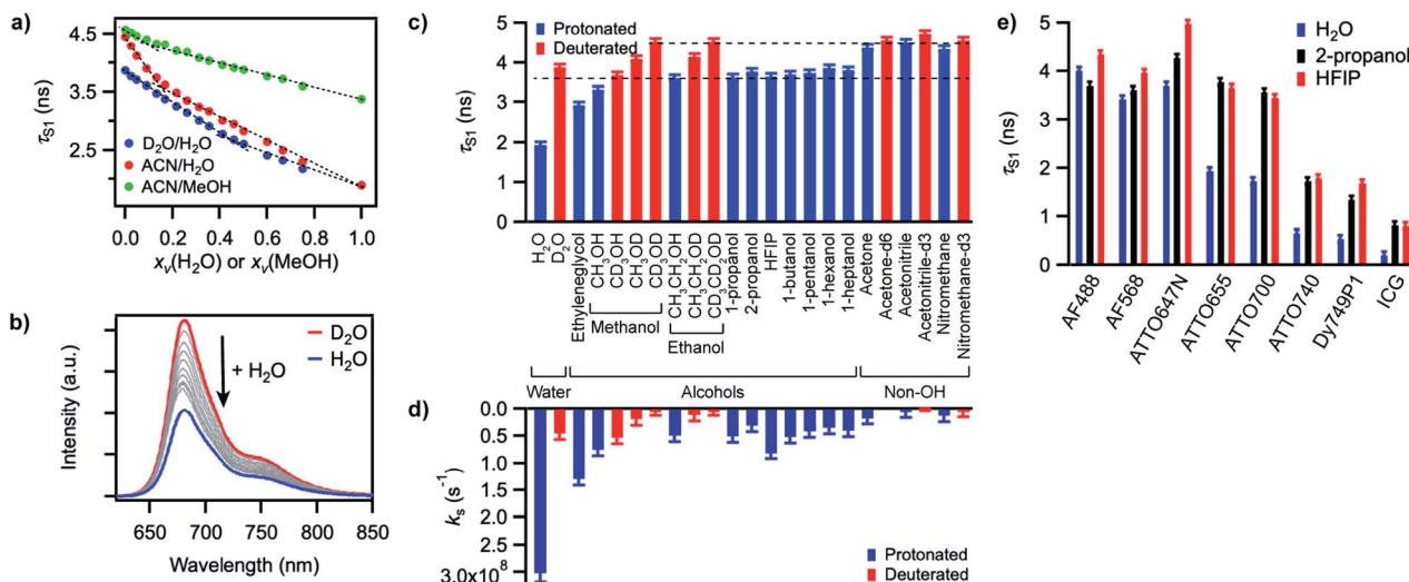
Fig. 3 (a) Excited-state lifetime of ATTO655 in \text{D}_2\text{O}/\text{H}_2\text{O} , \text{ACN}/\text{H}_2\text{O} , or \text{ACN}/\text{MeOH} mixtures as a function of the volume fraction x_v of \text{H}_2\text{O} or \text{MeOH} . Dashed lines serve as guide to the eye to emphasize deviation of the curves from linearity. (b) Evolution of the fluorescence spectrum of ATTO655 in \text{D}_2\text{O} upon addition of increasing amounts of \text{H}_2\text{O} (at constant dye absorbance). The red curve corresponds to the fluorescence spectrum in pure \text{D}_2\text{O} and the blue curve in pure \text{H}_2\text{O} . (c) Excited-state lifetime of ATTO655 in various protonated (blue) and partially or fully deuterated (red) solvents. The two dashed lines indicate the lifetime levels observed in alcohols (lower) and in other non-alcoholic polar solvents (upper). (d) Solvent-assisted quenching rate constant k_s determined for ATTO655 in the same solvents as in (c), with the assumption k_{\text{nr}} = 0 in acetonitrile- \text{d}_3 . (e) Excited-state lifetime of various fluorophores in \text{H}_2\text{O} , 2-propanol, and HFIP. The similarity of the lifetime values in 2-propanol and HFIP indicates that the H-bond strength does not significantly influence the fluorescence quenching process. All error bars reflect uncertainties on the lifetime measurements.
