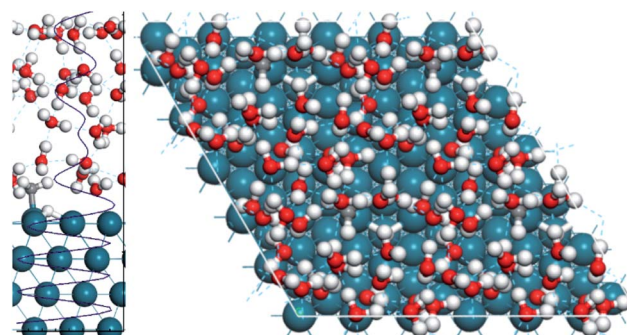
Fig. 3 Snapshot of the \text{H}_2\text{O}/\text{Pd}(111) interface with activated methane on the surface after 50 ps of simulation. A side view is shown on the left with the density profile of the last 10 ps of the simulation superimposed, where the average density of water is 1.0 \text{ kg m}^{-3} . The layers of water formed in solution are demonstrated. A top view is shown using a (2 \times 2) supercell of the p(3 \times 3) unit cell, showing the water structure in the unit cell.
