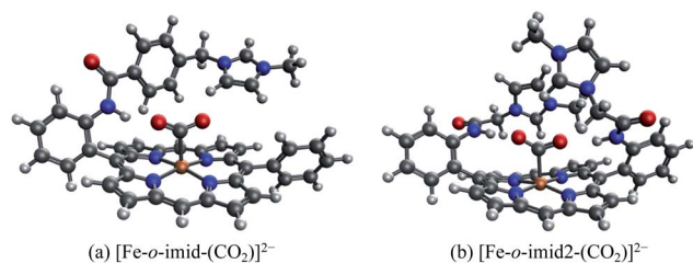
Fig. 12 Optimized geometries for (a) [\text{Fe-}o\text{-imid-(CO}_2\text{)}]^{2-} , which carries one methylimidazolium-containing group that was reported in ref. 98, and (b) [\text{Fe-}o\text{-imid2-(CO}_2\text{)}]^{2-} , which carries two modified methylimidazolium-containing groups.
