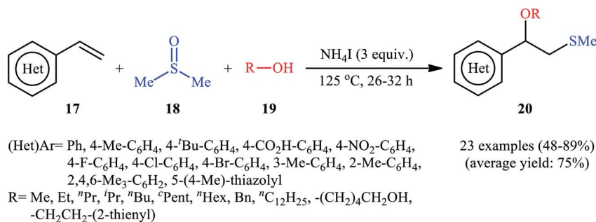
Scheme 7 Synthesis of \beta -alkoxy methyl sulfides 20 through the \text{NH}_4\text{I} -mediated three-component coupling alkenes 17 , dimethyl sulfoxide 18 and alcohols 19 .
