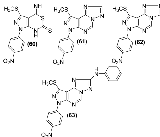
Fig. 15 Chemical structures of selected pyrazolo [3,4- d ] pyrimidines (60–63).
