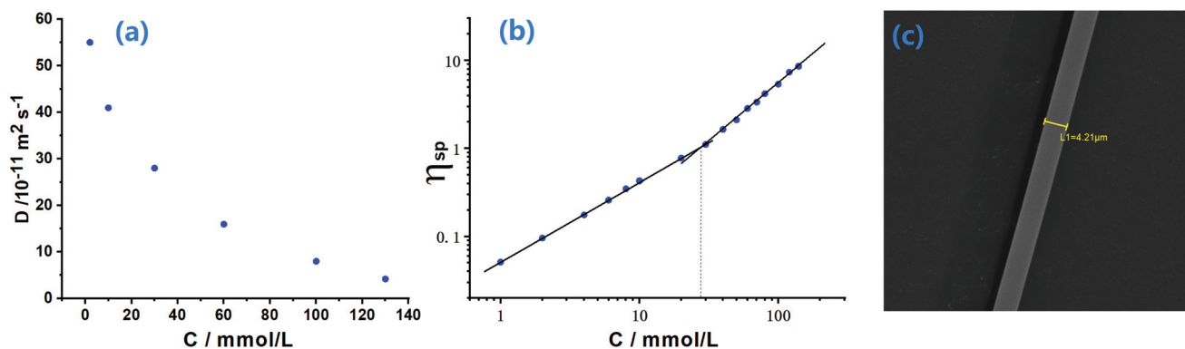
Fig. 4 (a) Diffusion coefficient of M1 + M2 + M3 + M4 + \text{Zn(OTf)}_2 against the concentration of M1 (600 MHz, 293 K); (b) specific viscosity of M1 + M2 + M3 + M4 + \text{Zn(OTf)}_2 against the concentration of M1. Molar ratio: M1 : M2 : M3 : M4 : \text{Zn(OTf)}_2 = 2 : 2 : 1 : 1 : 2 ; (c) SEM image of a rodlike fiber drawn from a highly concentrated solution of M1 + M2 + M3 + M4 + \text{Zn(OTf)}_2 .
