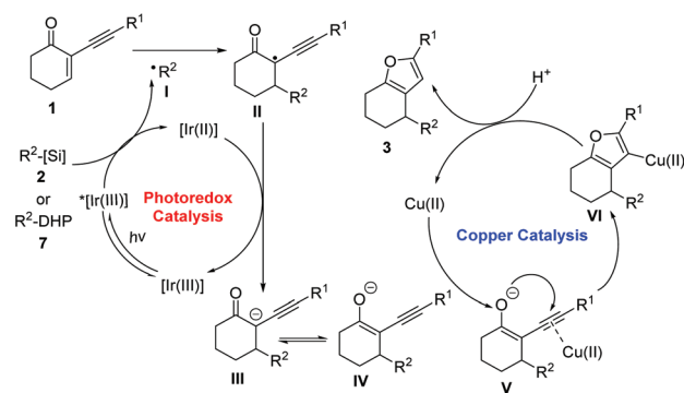
Scheme 5 Proposed mechanistic pathway.
