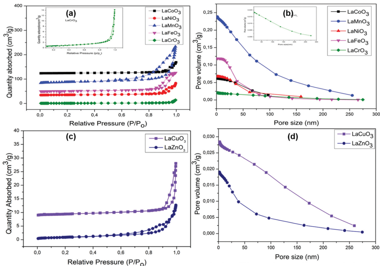
Fig. 5 Plots of (a) nitrogen adsorption–desorption isotherm curves (b) pore volume versus pore size for \text{LaMO}_3 ( M = \text{Co}, \text{Ni}, \text{Mn}, \text{Fe}, \text{Cr} ) (c) nitrogen-desorption isotherm curves and (d) pore volume versus pore size for \text{LaMO}_3 ( M = \text{Cu}, \text{Zn} ).
