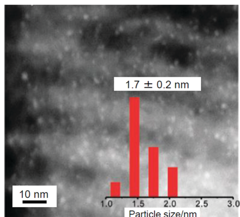
Fig. 20 STEM image of \text{Au}_{144} NCs (1.1 wt% Au) loaded on \text{CuO-EP-FDU-12} after calcination at 300\text{ }^{\circ}\text{C} and size distribution of Au NCs. Reproduced with permission from ref. 234. Copyright 2012 Royal Society of Chemistry.
