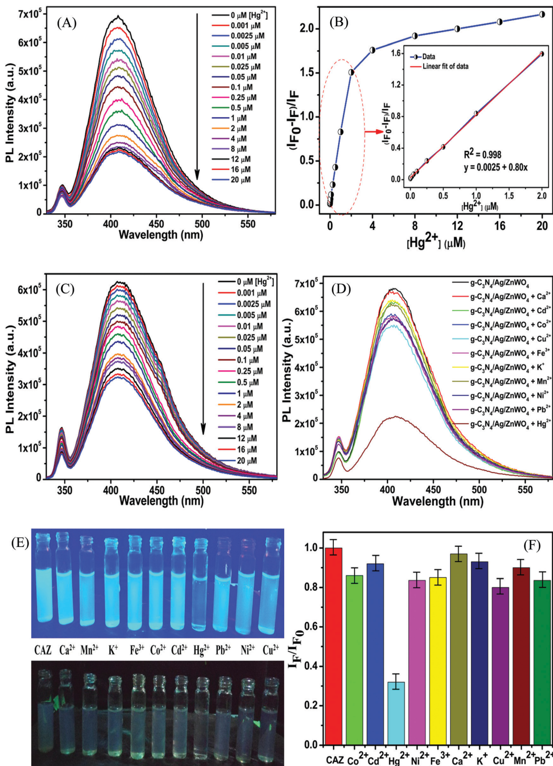
Fig. 7 (A) and (C) PL intensity responses of g\text{-C}_3\text{N}_4/\text{Ag}/\text{ZnWO}_4 in phosphate buffer (pH = 7.2) and tap water, respectively on the addition of different amounts of \text{Hg}^{2+} , \lambda_{\text{ex}} = 310 nm, (B) calibration curve of g\text{-C}_3\text{N}_4/\text{Ag}/\text{ZnWO}_4 for the detection of \text{Hg}^{2+} (inset is a linear plot of relative intensity vs. conc. of \text{Hg}^{2+} ), (D) PL emission of g\text{-C}_3\text{N}_4/\text{Ag}/\text{ZnWO}_4 in the presence of different metal ions individually ( \lambda_{\text{ex}} = 310 nm, [\text{M}^{n+}] = 10 \mu\text{M} ), (E) photographic image of g\text{-C}_3\text{N}_4/\text{Ag}/\text{ZnWO}_4 in phosphate buffer under 365 nm light (upper panel) and white light in the presence of different metal ions (10 \mu\text{M} ) (lower panel), and (F) bar diagram of the relative PL emission intensities ( I_F/I_{F_0} ) of g\text{-C}_3\text{N}_4/\text{Ag}/\text{ZnWO}_4 in the presence of various metal ions (10 \mu\text{M} ).
