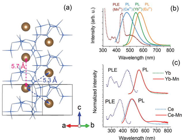
Fig. 7 \text{Ca-}\alpha\text{-SiAlON} crystal structure depicting \text{Ca-}\text{Ca} separation (a); spectral overlap of \text{Mn}^{2+} absorption (dotted line) with emissions (solid lines) of \text{Eu}^{2+} , \text{Yb}^{2+} and \text{Ce}^{3+} donor ions (b); and normalized PL–PLE spectra of \text{Yb}^{2+} and \text{Ce}^{3+} singly doped with respective \text{Mn}^{2+} codoped \text{Ca-}\alpha\text{-SiAlON} at 300 K (c). The doping concentration for \text{Yb}^{2+} and \text{Ce}^{3+} was 0.5 at%, and for \text{Mn}^{2+} was 10 at%. The excitation and emission wavelengths for PL and PLE measurements were 412 nm and 545 nm, respectively for \text{Yb}^{2+} -doped samples, and 375 nm and 495 nm for \text{Ce}^{3+} -doped samples, respectively.
