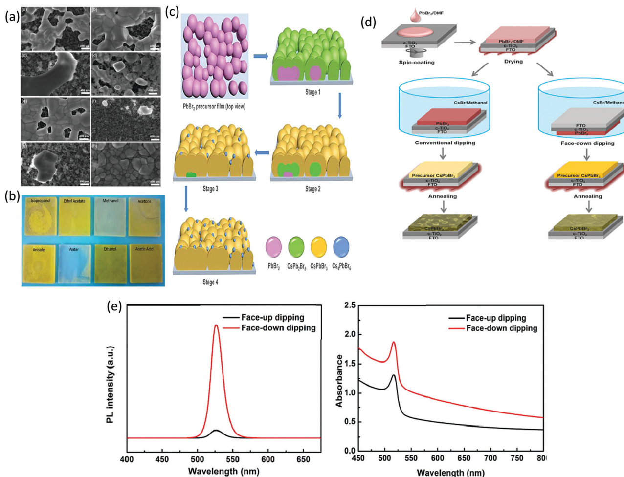
Fig. 7 (a) SEM micrographs of the Cs–Pb–Br films prepared using various solvent dropping methods. (b) The photographs of the Cs–Pb–Br films fabricated from \text{PbBr}_2/(\text{PEG} + 40\% \text{ GBL}) using various solvent dropping methods. Reproduced with permission ref. 122. Copyright 2020, Wiley-VCH. (c) Representation of the conversion mechanism from the \text{PbBr}_2 precursor film to the Cs–Pb–Br films in the methanol-based two-step process. Reproduced with permission ref. 123. Copyright 2020, Elsevier Ltd. (d) Multi-step solution method via the dipping process of the \text{CsPbBr}_3 film (e) UV-vis absorption and PL spectra of the as-prepared \text{CsPbBr}_3 films. Reproduced with permission ref. 117. Copyright 2018, American Chemical Society.
