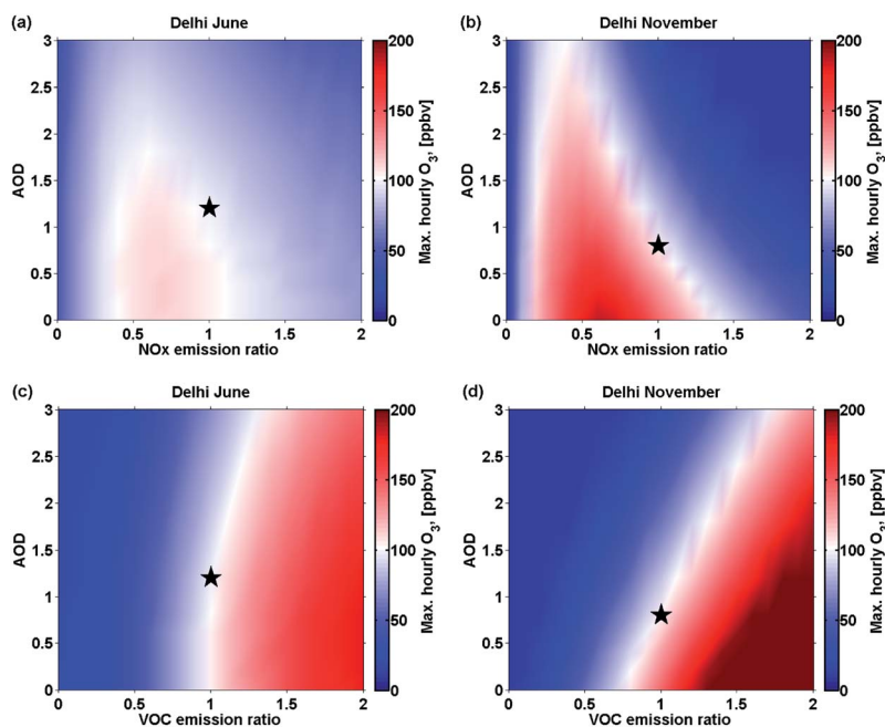
Fig. 4 The impact of AOD on the non-linear VOC- \text{NO}_x -ozone relationship in Delhi. (a) Impact on relationship between \text{NO}_x and ozone in summer (June), (b) between \text{NO}_x and ozone in winter (November), (c) between VOC and ozone in summer, and (d) between VOC and ozone in winter. Current conditions are marked by a black star.
