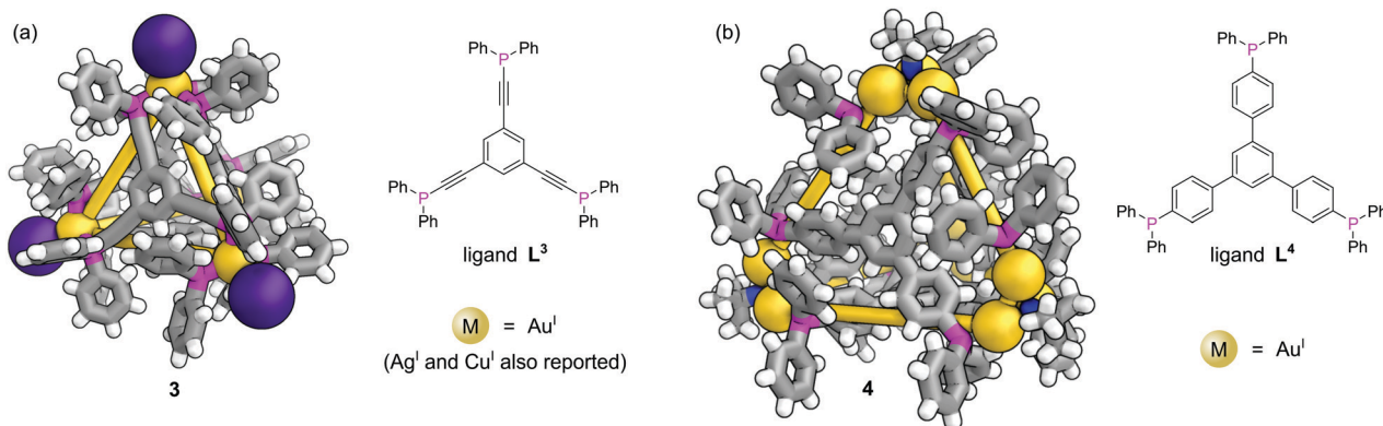
Fig. 3 Structural metal–phosphine coordination to hold together metal–organic cages: (a) M_4L_4 tetrahedral metal organic cage 3 formed with \text{Au}^{\text{I}} . \text{Ag}^{\text{I}} and \text{Cu}^{\text{I}} congeners also reported; (b) tetrahedral metal–organic cage 4 , where each vertex consists of a \text{Au}_3 triangle held together by a \mu_3\text{-NtBu}^{2-} unit and aurophilic interactions. Colours: C grey, H white, Au gold (shown as spheres), I dark purple (shown as spheres), N blue, P magenta.
