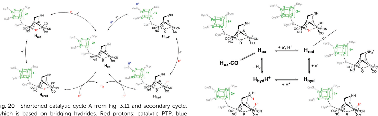
Fig. 21 Schematic representation of the catalytic cycle of [\text{FeFe}] -hydrogenase, based on the states observed under whole-cell conditions including the protonated hydride species ( \text{H}_{\text{hyd}}\text{H}^+ ). Figure and caption from ref. 35.
