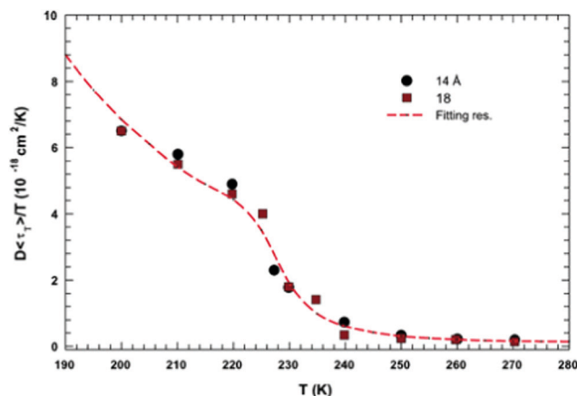
Fig. 2 The quantity D \langle \tau_T \rangle / T as a function of T . Dots and squares represent its values coming from the experimental data of D and \tau_T in samples with diameters of 14 and 18 Å, respectively. The dotted line represents the same quantity obtained by using the fitting values obtained from the data reported in Fig. 1. Reprinted from ref. 55. Copyright (2006) National Academy of Sciences, U.S.A.
